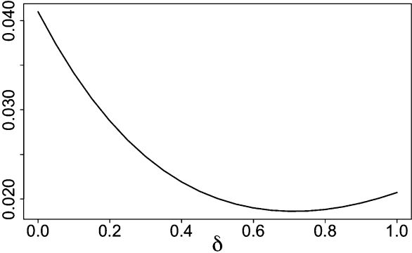
Fig. 61 \mathbb{E}\theta(\mathbb{Z}_n) for Design S2: d = 20, n = 1024
