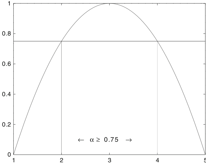
Fig. 1 The \alpha -cut \alpha \geq 0.75 for Example 4
