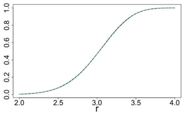
Fig. 10 P_{U,\delta,0,r} and approximations: d = 20, seed = 10
