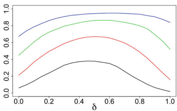
Fig. 58 C_d(\mathbb{Z}_n, r) for Design S2: d = 50, n = 1024, r from 0.11 to 0.14 increasing by 0.01
