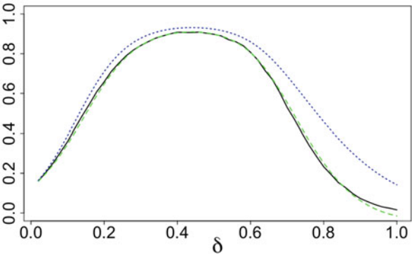
Fig. 21 Design 2a: C_d(\mathbb{Z}_n, r) and approximations; d = 10, \alpha = 0, n = 128
