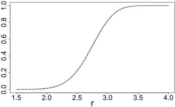
Fig. 4 P_{U,\delta,\alpha,r} and approximations: d = 20, \alpha = 0.5
