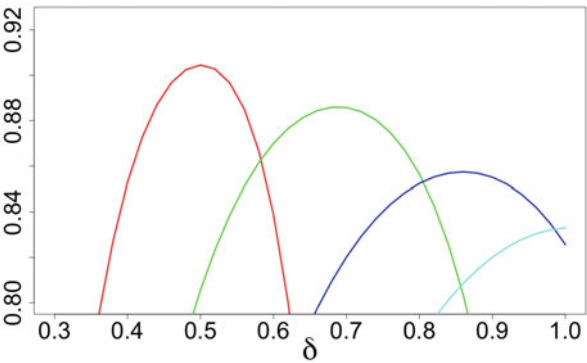
Fig. 29 d = 10, n = 512, r = 1.228
