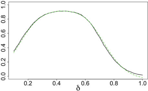
Fig. 25 Design 2b: C_d(\mathbb{Z}_n, r) and approximation (27); d = 10, n = 128
