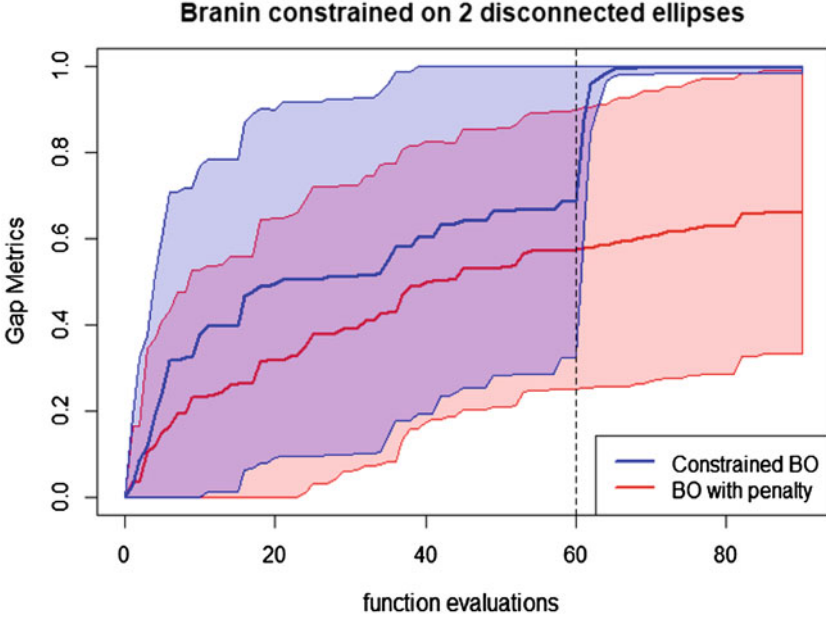
Fig. 10 The figure represents the gap metric values over 30 independent runs of SVM-CBO and BO with penalty on constrained Branin test function constrained to two ellipses. The main remark in this result comparison is the relevant shift, in terms of gap metric, that the SVM-CBO approach encountered when passed in its second phase, pointed by vertical black dashed line, that means the optimization phase
