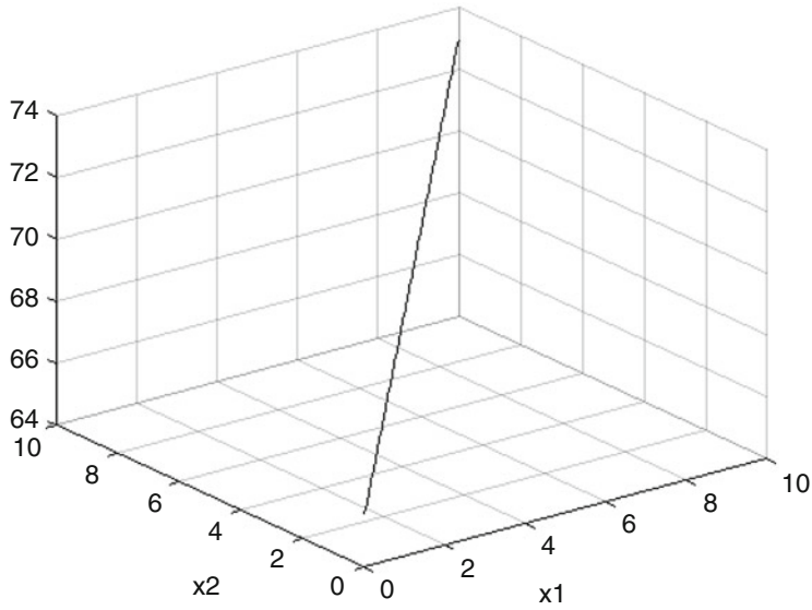
Fig. 16 Central Federal District output according to variables x_1 and x_2
