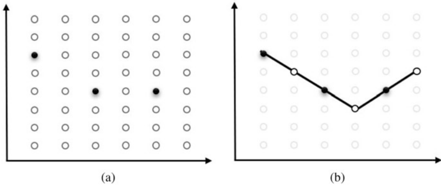
Fig. 3 The sample of points collected so far will not say anything about the values of the function in other regions (case a ). For a given subclass of functions, for example convex (Case b ), those algorithms that can take advantage of this structure will perform better than others
