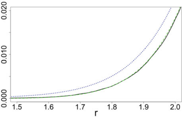
Fig. 8 P_{U,\delta,\alpha,r} and approximations: d = 20, \alpha = 1
