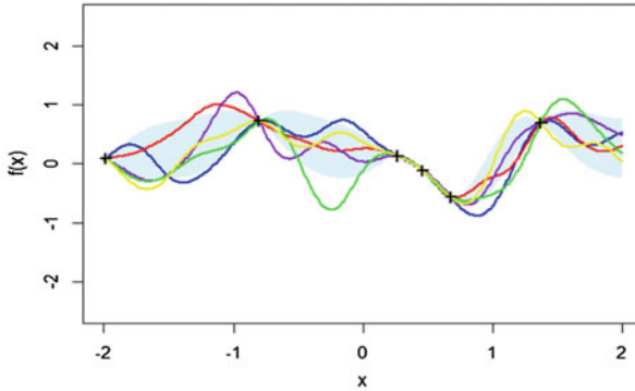
Fig. 2 Sampling from prior vs sampling from posterior (for the sake of simplicity, we consider the noise-free setting) [Source: [6]]
