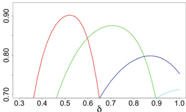
Fig. 30 d = 10, n = 1024, r = 1.13
