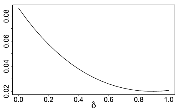
Fig. 59 \mathbb{E}\theta(\mathbb{Z}_n) for Design S1: d = 20, n = 1024
