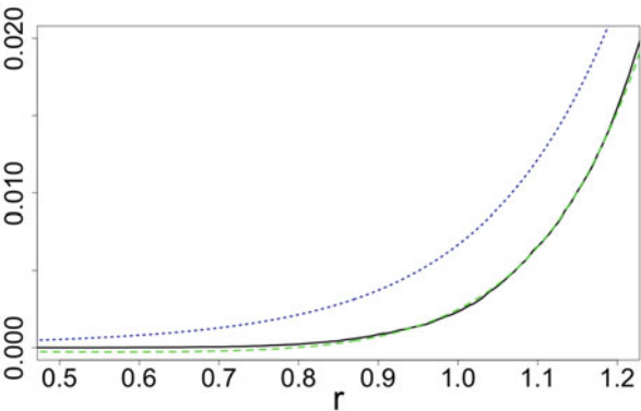
Fig. 6 P_{U,\delta,\alpha,r} and approximations: d = 10, \alpha = 1
