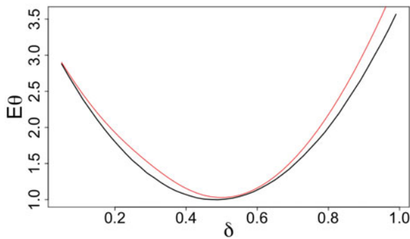
Fig. 42 \mathbb{E}\theta(\mathbb{Z}_n) and approximation (35): d = 10, n = 500
