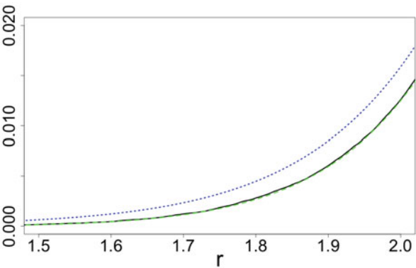
Fig. 7 P_{U,\delta,\alpha,r} and approximations: d = 20, \alpha = 0.5
