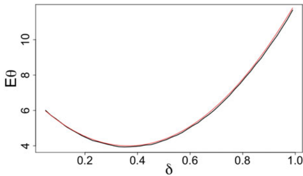
Fig. 43 \mathbb{E}\theta(\mathbb{Z}_n) and approximation (35): d = 20, n = 500
