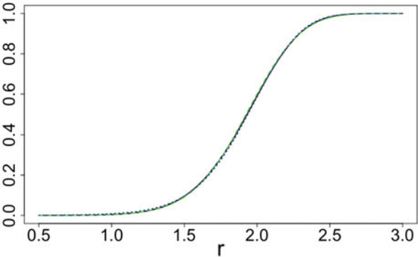
Fig. 3 P_{U,\delta,\alpha,r} and approximations: d = 10, \alpha = 0.5
