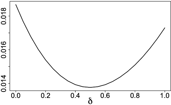
Fig. 62 \mathbb{E}\theta(\mathbb{Z}_n) for Design S2: d = 50, n = 1024
