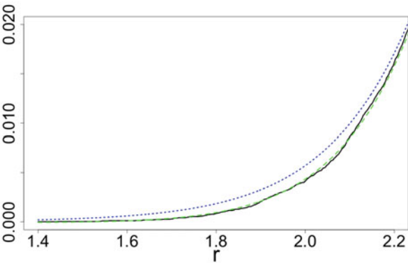
Fig. 13 P_{U,\delta,0,r} and approximations: d = 20, seed = 10
