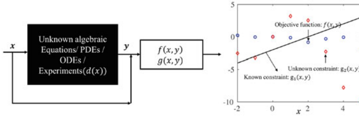
Fig. 1 Illustration of a BBO problem. The values of y are obtained by fixing x , which are then used to compute black-box objective function (blue circles) and the unknown constraints (red diamonds). The known constraints (black solid line) are functions of only decision variables
