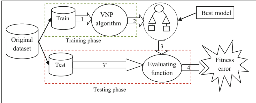
Fig. 11 Learning process schema
