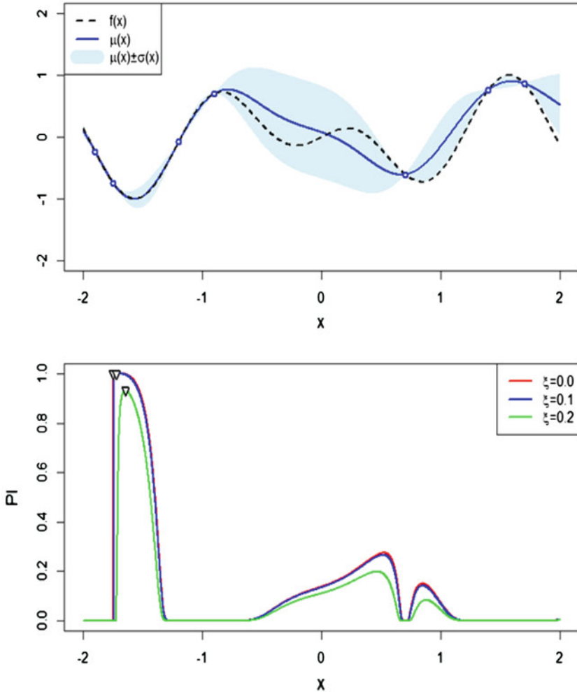
Fig. 5 GP trained depending on 7 observations (top), PI with respect to different values of \xi and max values corresponding to the next point to evaluate (bottom) [Source: [6]]
