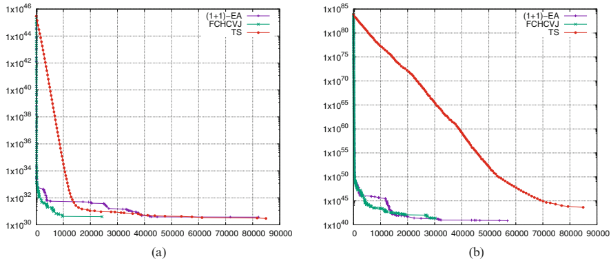
Fig. 2 Minimization of the objective function (17) on Trivium and Grain_v1 by (1+1)-EA, FCHCVJ, and TS. (a) Grain_v1. (b) Trivium
