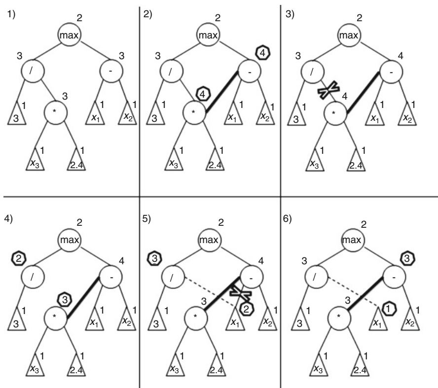
Fig. 8 An example of ETT move in AP tree: from the expression T = \max \left\{ \frac{3}{x_3 * 2.4}; x_1 - x_2 \right\} , the neighboring T' = \max \left\{ \frac{3}{x_1}; x_3 * 2.4 - x_2 \right\} is obtained
