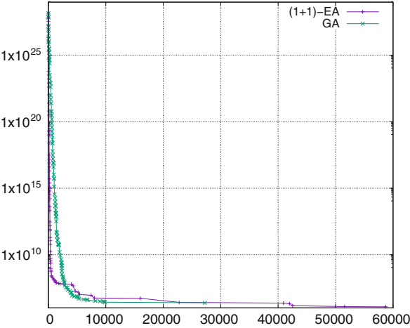
Fig. 1 Minimization of the objective function (14) on ASG-96 by (1+1)-EA and GA
