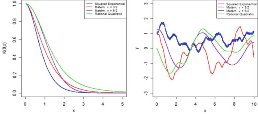
Fig. 3 Value of four different kernels with x moving away from x' = 0 (left) and four samples from GP prior, one for each kernel considered (right). The value of the characteristic length scale is l = 1 for all the four kernels; \alpha of the RQ kernel is set to 2.25 [Source: [6]]
