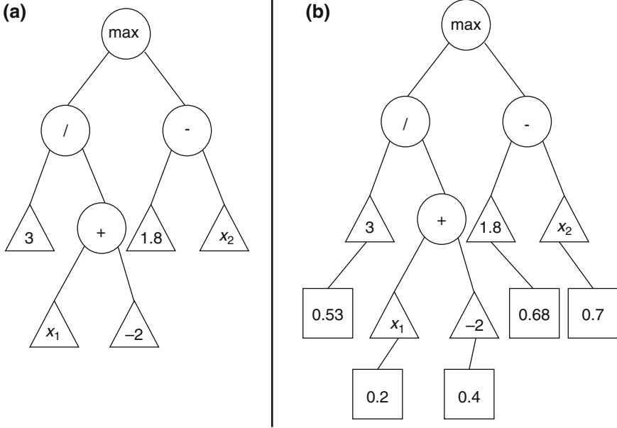
Fig. 2 (a) Solution presentation in GP; (b) Solution representation in VNP
