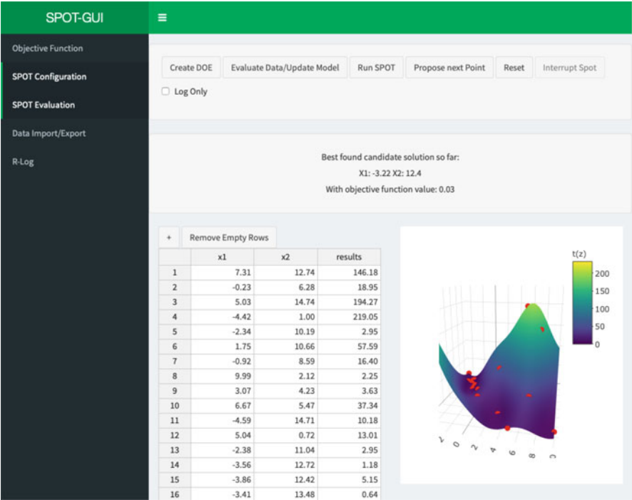
Fig. 2 Screenshot of the spotGUI software during the tuning process. Using buttons on the top, the user can execute commands in SPOT. From left to right, it is possible to create a DOE and evaluate given candidate solutions. The “Run SPOT” button starts the SPO procedure and uses the configured budget for tuning. With “Propose next Point,” a single iteration of SPO is executed, creating a new design point. The tuning process can be reset, and SPOT can be interrupted during the tuning procedure. The spotGUI output can be seen on the lower half of the image. An overview of all candidate solutions is available with an interactive 3D plot of the modeled parameter landscape. Red dots in the landscape mark the evaluated candidates
