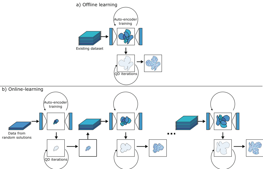
Fig. 3 Different approaches to learning the behavioral descriptor. (a) An existing dataset can be used to train an auto-encoder (offline) and define a latent representation of the data. This latent space is then used as the behavioral descriptor space and a QD algorithm can build a collection of solutions filling this latent space. (b) Alternatively, the learning of the behavioral descriptor can be achieved during the QD optimization process. Starting from randomly generated solutions, the auto-encoder is trained and the produced latent space used as a behavioral descriptor. Then, the several QD steps are executed to generate new solutions in the latent space, which increase the amount of data available to train the auto-encoder. The training of the auto-encoder is then extended and the process can repeat until convergence of both the QD algorithm and the auto-encoder
