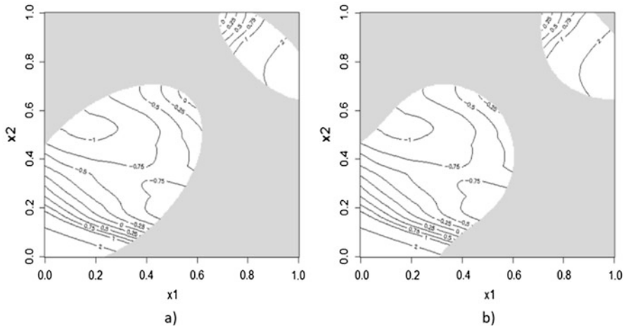
Fig. 8 Panels (a) and (b) both represent the BO-based surrogate function with LCB acquisition function. The constrained test function used is the Branin test function, and it is defined in X = [0, 1]^2 . Also, two nonlinear constraints are defined by two ellipses on this test function by Candelieri and Archetti [14]. Panel (a) represents the surrogate function with real constraints that define the infeasible region (grey region). Instead, panel (b) represents the surrogate function with an estimation of constraints provided by SVM classifier inside of the SVM-CBO approach
