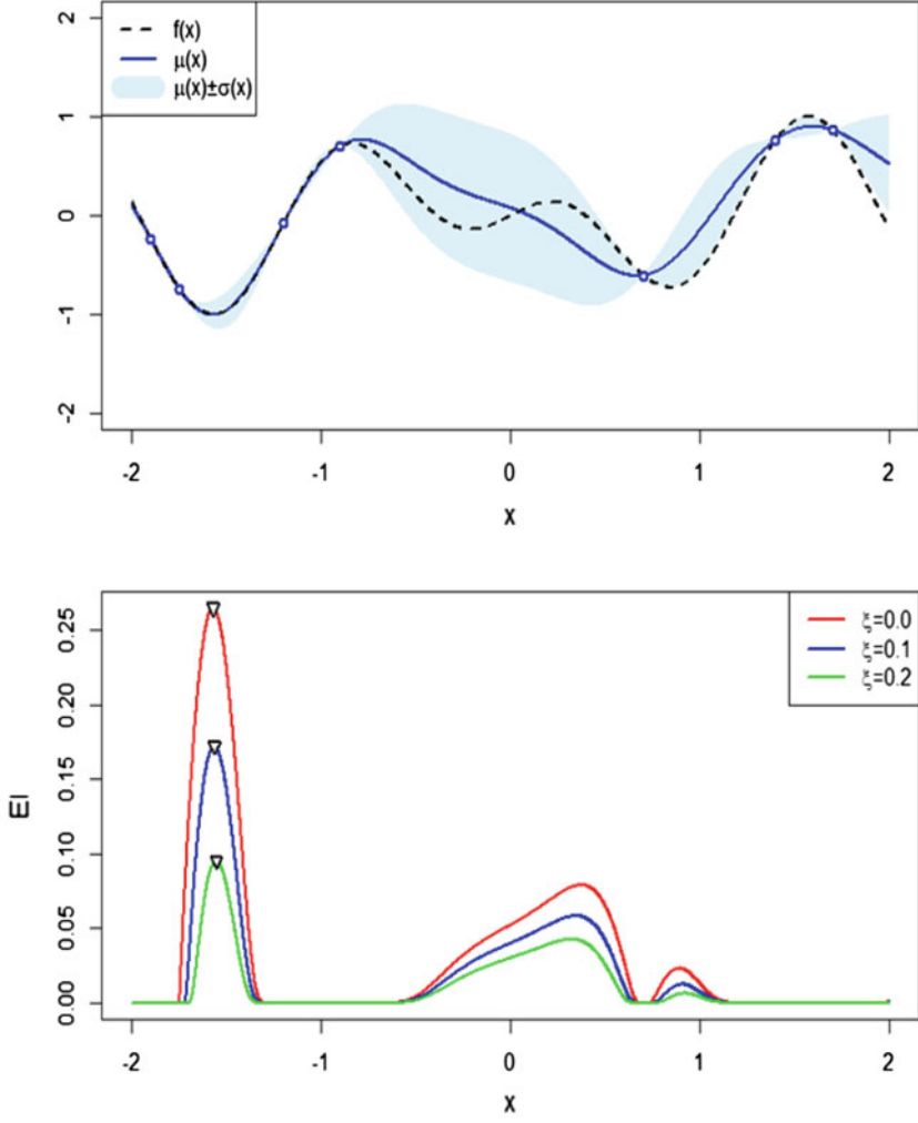
Fig. 6 GP trained depending on 7 observations (top), EI with respect to different values of \xi and max values corresponding to the next point to evaluate (bottom) [Source: [6]]
