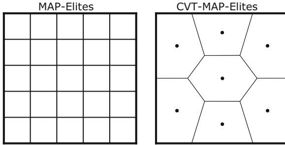
Fig. 2 MAP-Elites (left) partitions the feature space using a number of bins (25 in this example), k , that is computed by the number of discretization intervals per dimension requested by the user (i.e., k = \prod_{i=1}^d n_i , where d is the dimensionality of the feature space and n_i is the discretization interval of dimension i ). CVT-MAP-Elites (right) has explicit control over the number of bins (7 in this example) irrespective of the dimensionality of the feature space. Figure taken from [78]
