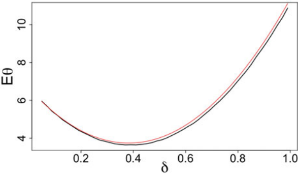
Fig. 44 \mathbb{E}\theta(\mathbb{Z}_n) and approximation (35): d = 20, n = 1000
