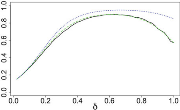
Fig. 15 Design 1: C_d(\mathbb{Z}_n, r) and approximations; d = 10, \alpha = 0.5, n = 128
