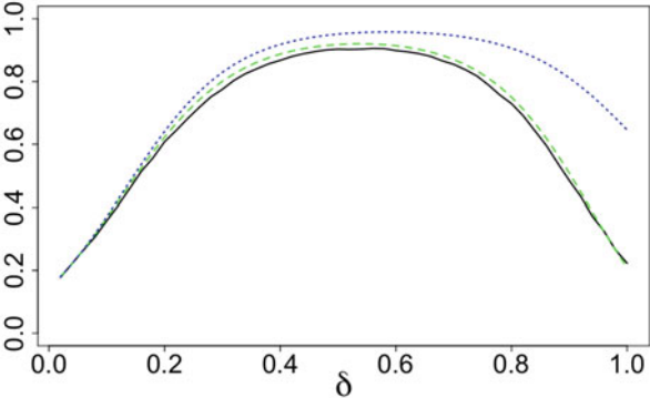
Fig. 17 Design 1: C_d(\mathbb{Z}_n, r) and approximations; d = 20, \alpha = 0.5, n = 512
