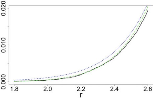
Fig. 14 P_{U,\delta,0,r} and approximations: d = 20, seed = 15
