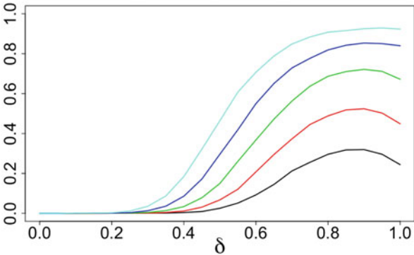
Fig. 53 C_d(\mathbb{Z}_n, r) for Design S1: d = 20, n = 1024, r from 0.13 to 0.17 increasing by 0.01
