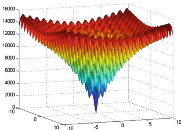
Fig. 5 Polypeptide molecular potential energy has a funnel-like geometry. Here is a simplified 3D example
