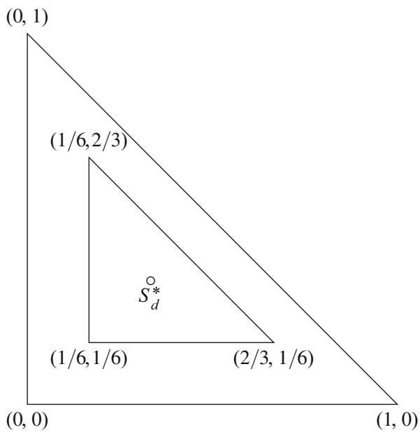
Fig. 50 S_d and S_{d,2}^{(\delta)} with d = 2 and \delta = 0.5
