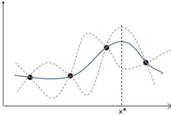
Fig. 4 Bayesian optimization. Data points are shown as black dots. The GP modeled distribution has a mean shown by the blue line that fits the data, and a standard deviation represented here by the red dotted lines. Here x^* represent the next point to explore since maximum improvement is expected
