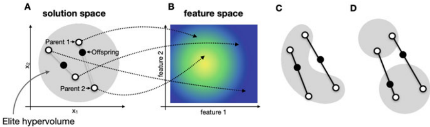
Fig. 4 Concept of the elite hypervolume [75]. (a)–(b) The elites of the feature space (b) occupy a very specific volume in the search space (a), here represented with a circle. If this volume is convex, then blending two elites creates a new elite. (c)–(d) If the elite hypervolume is not convex, then the blending is not guaranteed to generate a new elite, but it can still happen
