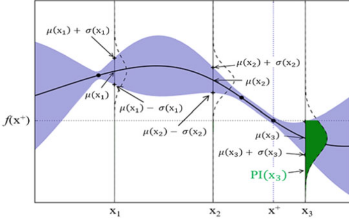
Fig. 4 A representation of probability of improvement [Source: [6]]
