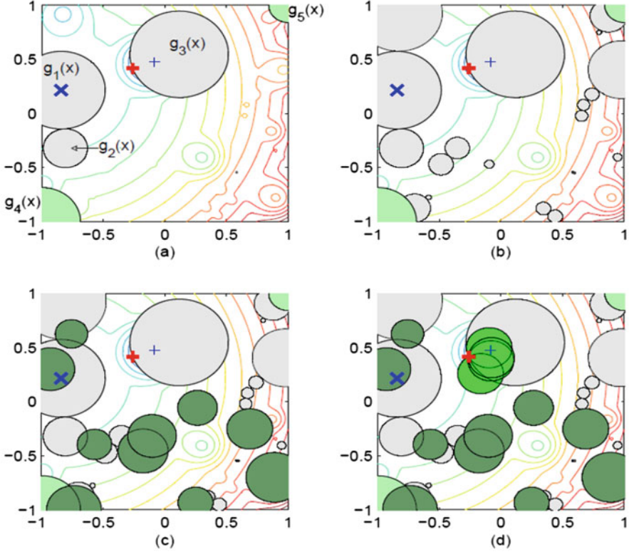
Fig. 11 Four examples of constrained objective functions generated through Emmental-type GKLS [70]. The objective function is the same, the set of constraints is different. The blue crosses are the global minimizers of the basis paraboloid functions, while the blue pluses are the global minimizers of the unconstrained problem. The red pluses are the global minimizers of the constrained problem. The infeasible regions are coloured according to the associated constraint type (grey for the first type, light green for the second, dark green for the third and bright green for the fourth one)
