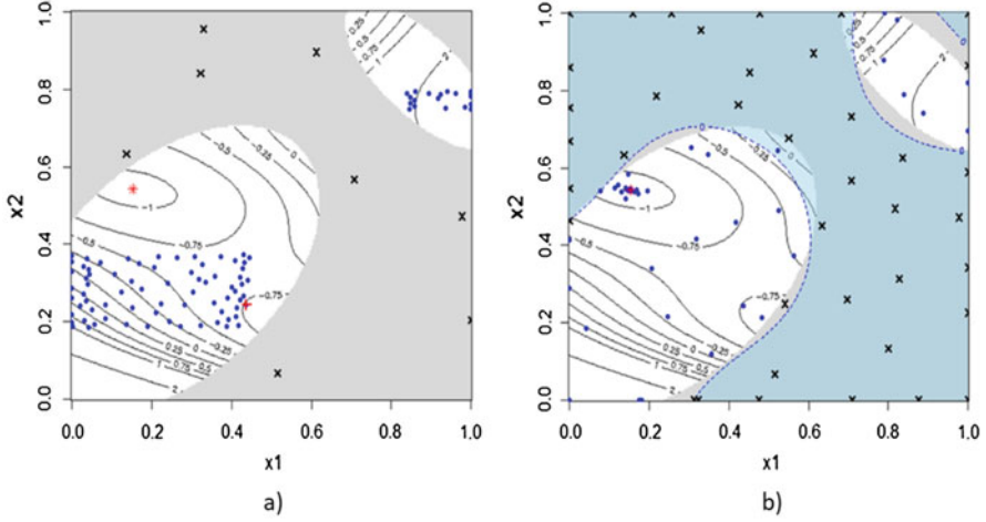
Fig. 9 Panels (a) and (b) represent the comparison between BO with penalty against SVM-CBO [14] on the test function of Fig. 8. In both panels, (a) and (b), the infeasible region (grey region) is defined by two ellipses, while the red star represents the feasible global minimizer, and the red plus represents the optimal minimum found by each approach. The black cross points represent non-computable points, and the blue points represent feasible function evaluations. In panel (b), it is also possible to see the estimated feasible region according to the SVM classifier. In panel (b), it is possible to notice that the optimal solution identified by SVM-CBO is the feasible global minimizer
