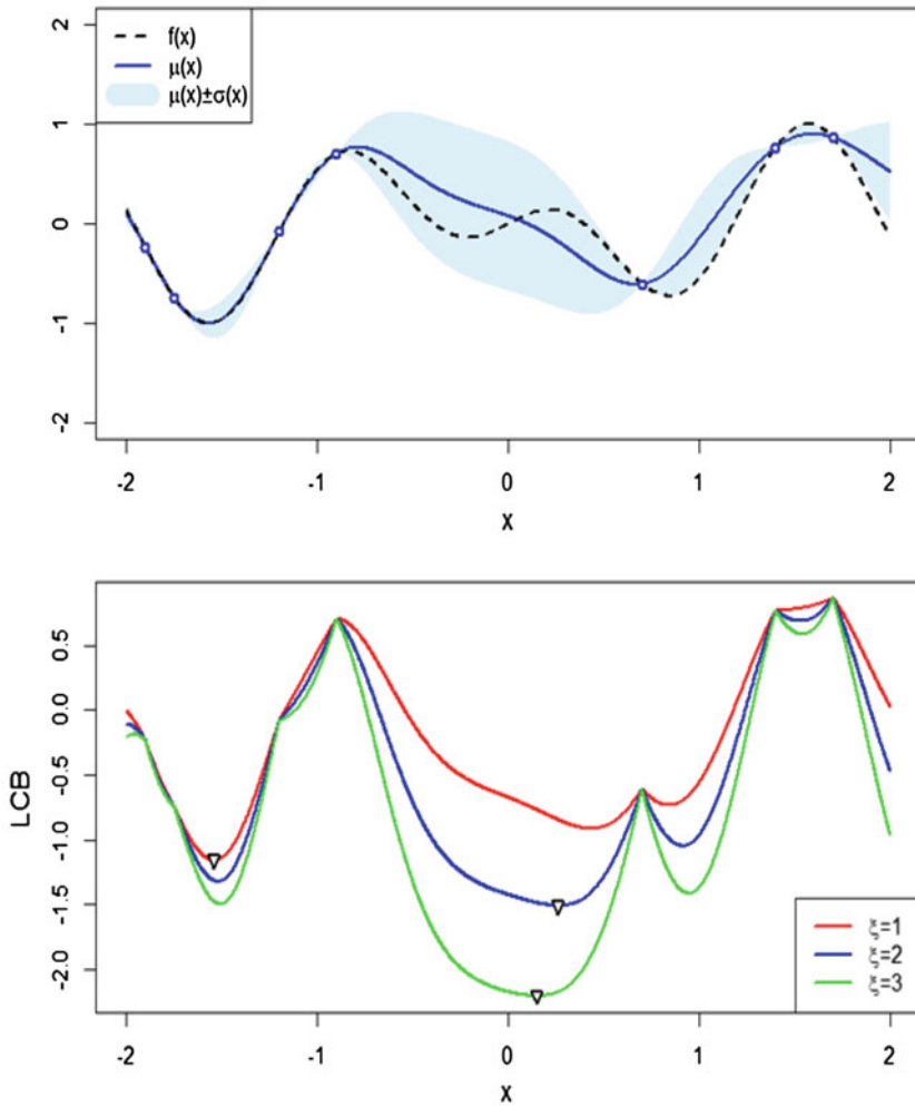
Fig. 7 GP trained depending on 7 observations (top), LCB with respect to different values of \xi and min values corresponding to the next point to evaluate (bottom). Contrary to the other acquisition function, LCB is minimized instead of maximized [Source: [6]]
