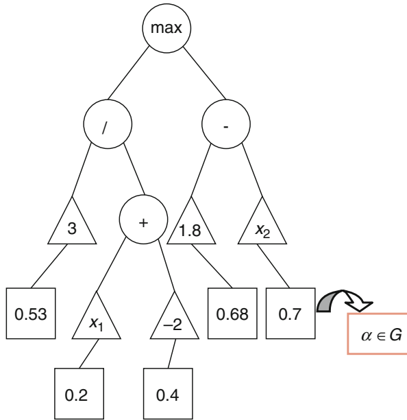
Fig. 6 Neighborhood structure N_3 : changing a parameter value
