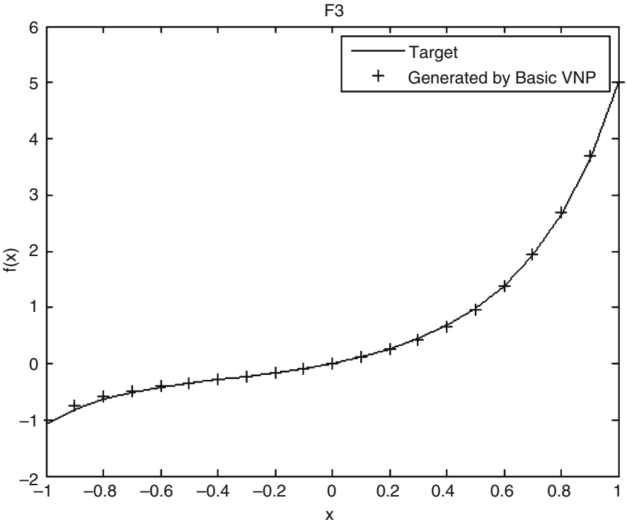
Fig. 9 Target and generated F3 functions obtained by Basic VNP
