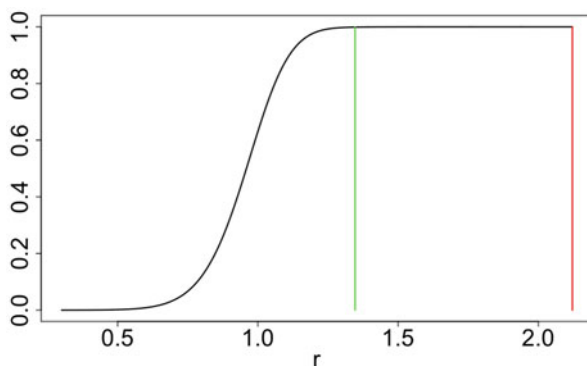
Fig. 1 C_d(\mathbb{Z}_n, r) with r_{0.999} and r_1 : d = 10 , \mathbb{Z}_n is a 2^{d-1} -factorial design with n = 2^{d-1}
