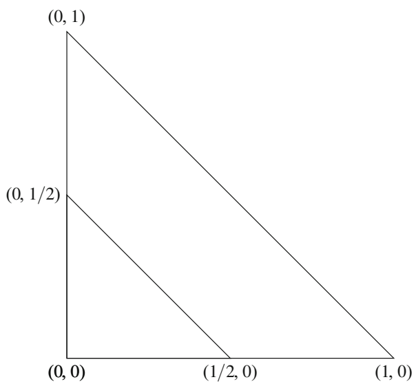
Fig. 49 S_d and S_{d,1}^{(\delta)} with d = 2 and \delta = 0.5
