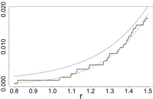
Fig. 12 P_{U,\delta,0,r} and approximations: d = 10, seed = 15
