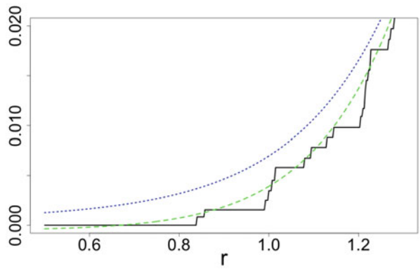
Fig. 11 P_{U,\delta,0,r} and approximations: d = 10, seed = 10
