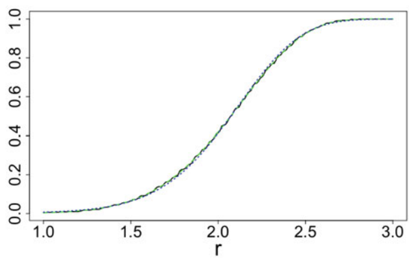
Fig. 9 P_{U,\delta,0,r} and approximations: d = 10, seed = 10
