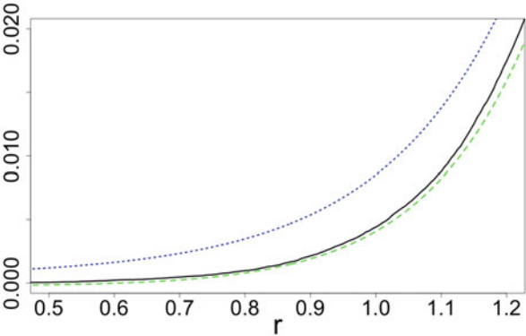
Fig. 5 P_{U,\delta,\alpha,r} and approximations: d = 10, \alpha = 0.5
