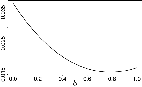
Fig. 60 \mathbb{E}\theta(\mathbb{Z}_n) for Design S1: d = 50, n = 1024
