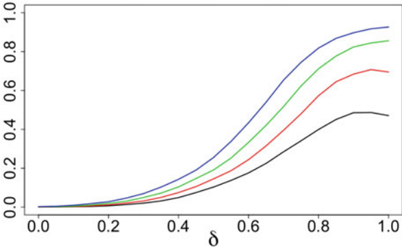
Fig. 51 C_d(\mathbb{Z}_n, r) for Design S1: d = 5, n = 128, r from 0.11 to 0.17 increasing by 0.02
