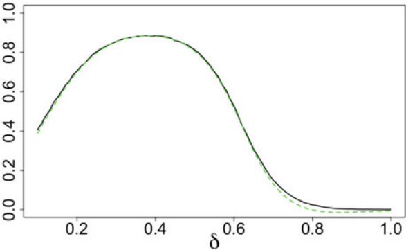
Fig. 27 Design 2b: C_d(\mathbb{Z}_n, r) and approximation (27); d = 20, n = 512
