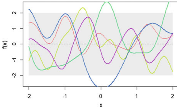
Fig. 1 Five different samples from the prior of a GP with Squared Exponential kernel as covariance function [Source: [6]]
